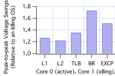
Fig. 12: Effect of microarchitectural events on supply voltage.
