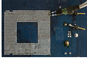
(a) Connecting to on-die voltage pins via a low impedance path using VCC_{sense} and VSS_{sense} .
