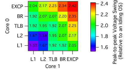
Fig. 13: Impact of microarchitectural event interference across cores.
