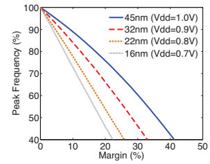
Fig. 2: Worst-case margins needed for noise are inefficient.
