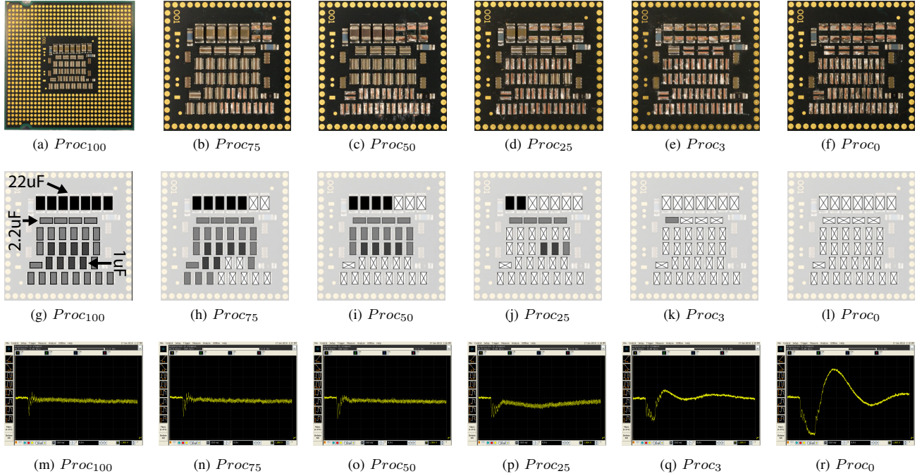
Fig. 5: (a)-(f) Land side of a Core2Duo™ processor, showing its package capacitors as we incrementally remove them to extrapolate voltage noise. (g)-(l) Capacitor values and the manner in which each chip is altered; white boxes with a cross correspond to removed capacitors. (m)-(r) Voltage droop response to the reset signal.
