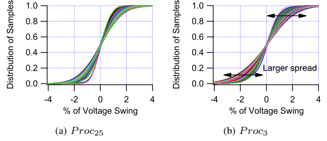
Fig. 9: Typical-case swings in future processors are increasingly more slanted compared to Proc 100 (see Fig. 7) as voltage noise grow.
