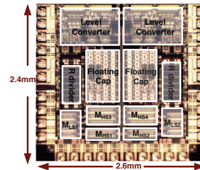
Fig. 10: Chip photograph for the power IC.
