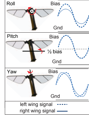
Fig. 3: Drive signals creates rotations in three axes.
