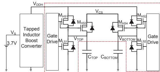
Fig. 5: The proposed actuator driver enables envelope tracking, dynamic common mode, and charge sharing to save power.
