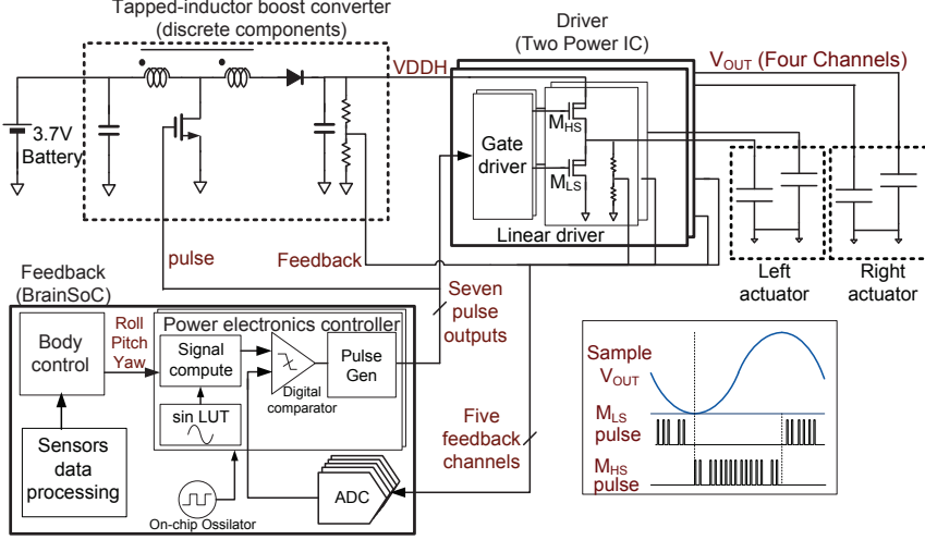
Fig. 2: A PEU design consists of two identical power ICs, a SoC and a off-chip boost converter.
