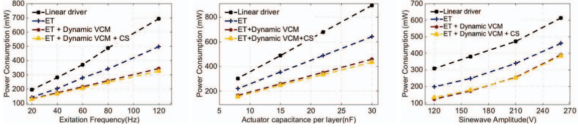
Fig. 9: Total power consumption scale with excitation frequency, actuator capacitance, and sinusoidal drive signal amplitude.
