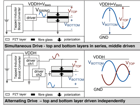
Fig. 4: There are two options to drive a bimorph PZT actuator. Simultaneous drive requires one driver connected to the middle layer. Alternating drive relies on two driver channels to generate out-of-phase sinusoids across the PZT layers with a grounded middle layer.
