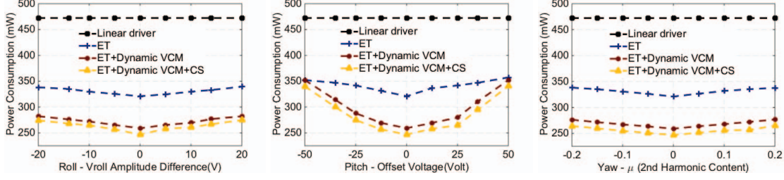
Fig. 8: The total power consumption changes depending on roll, pitch and yaw commands.
