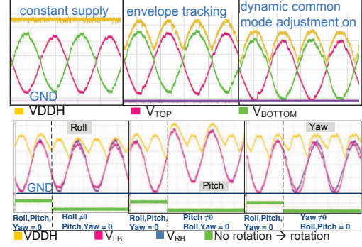
Fig. 7: Top row of oscilloscope waveforms of VDDH and top and bottom PZT drive signals demonstrate envelope tracking and dynamic common mode. Bottom row shows left and right driver waveforms for non-zero roll, pitch, and yaw rotation.
