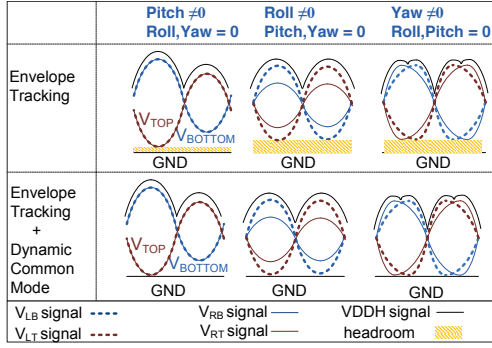
Fig. 6: Comparison between the roll, pitch, and yaw drive signals shows the adjustment to VBIAS and the common mode voltage while keeping differential voltage consistent for the simultaneous drive configuration.
