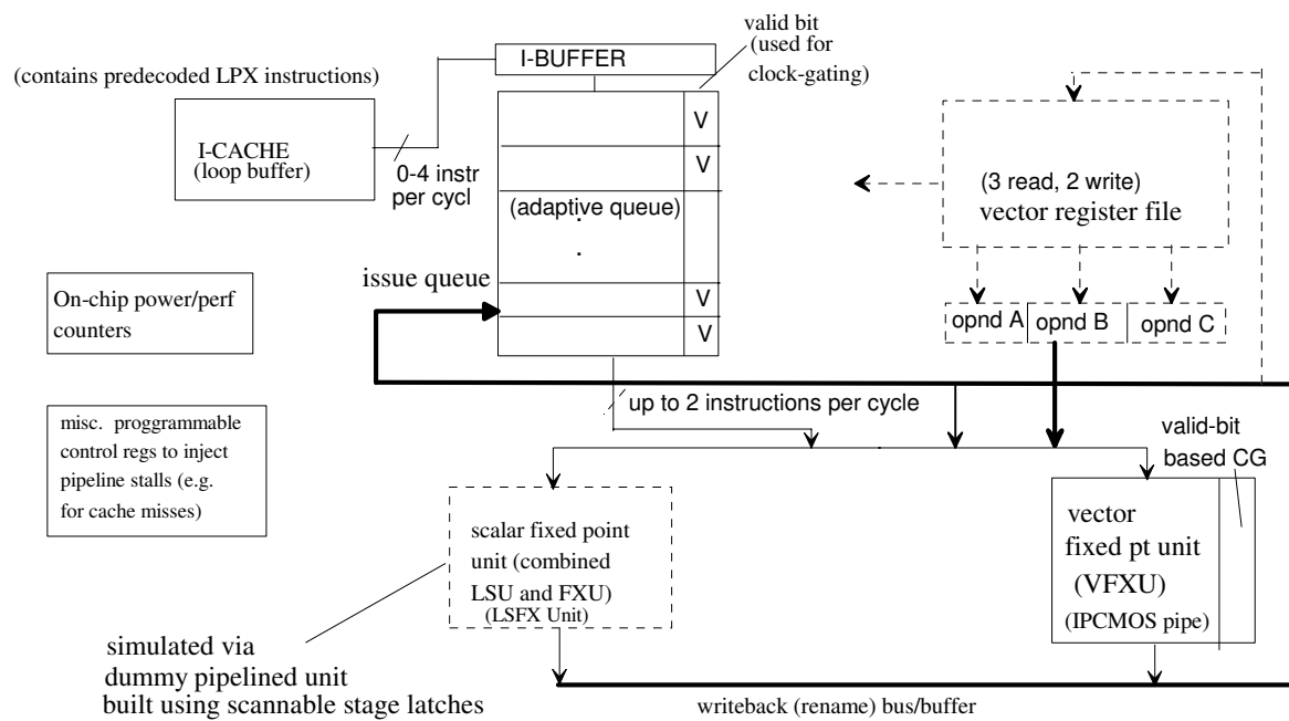
Figure 5. LPX Processor: High-Level Block Diagram
