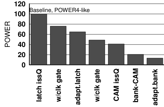
Fig. 9. Adaptive issue queue: power saving (generalized 8-issue super scalar model)
