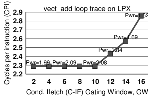
Fig. 8(b). Cond. ifetch in LPX: CPI vs. gating wind
