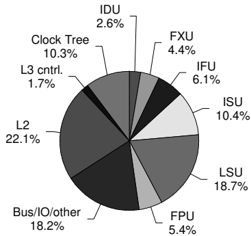
Fig. 1(a). Relative (unconstrained) unit-wise power
