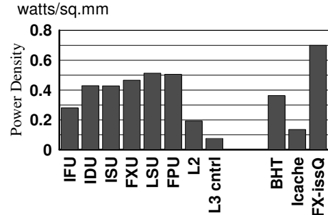
Fig. 2. Unconstrained power density profile
