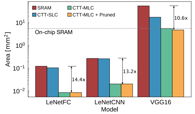
Figure 7: Area comparison for SRAM, CTT-SLC, and CTT-MLC for clustered encodings. Area for CTT-MLC with clustered and pruned encodings is also given (orange). The horizontal gray line indicates the memory area footprint from a recently published NN SoC [6], showing that our most optimized encoding enables VGG16 to fit on chip.
