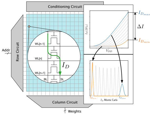
Figure 2: SPICE simulation for extracting the current distributions. The I_{Dmax} and I_{Dmin} values are based on measurement results, while the intermediate programmed levels are obtained from Monte Carlo simulations.
