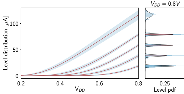
Figure 1: Measurements from a 16nm FinFET test chip we fabricated. The left plot shows the CTTs mean current and 2\sigma confidence intervals for different programmed levels as a function of V_{DD} . The right plot shows the distribution of the cell currents measured at V_{DD} = 0.8 V.
