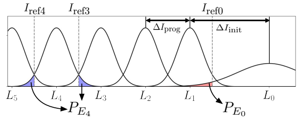
Figure 3: Example of the level current distributions showing fault probabilities for the initial level, L_0 , and one programmed level, L_4 .
