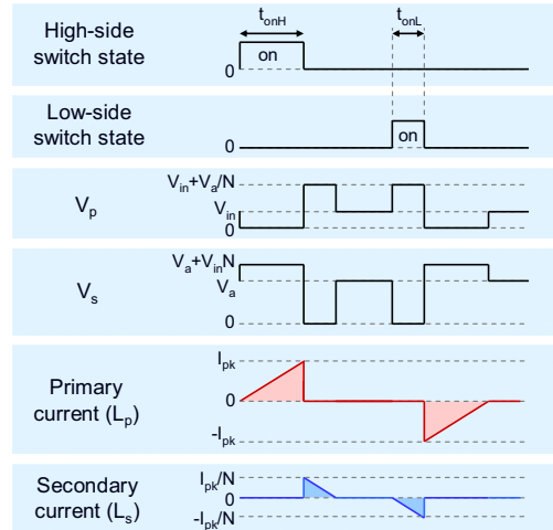
Fig. 8. Voltage and current waveforms during typical switching cycles for the bidirectional flyback converter.
