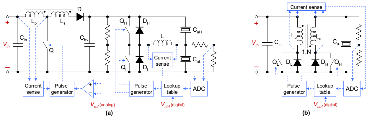
Fig. 10. Block diagrams of the dual-stage drive circuit (a), and single-stage drive circuit (b).
