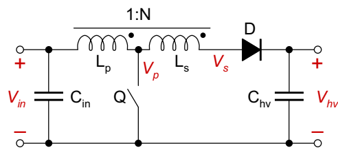
Fig. 3. Autotransformer boost converter.
