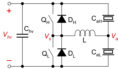
Fig. 5. Switching amplifier drive stage.
