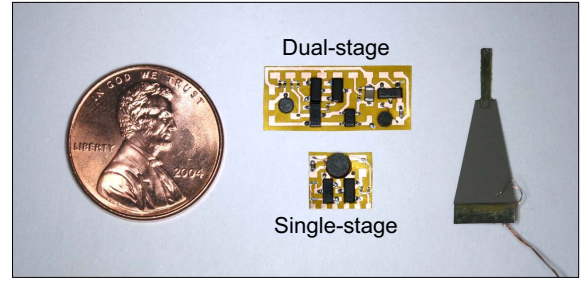
Fig. 9. Dual-stage and single-stage drivers (with external control) implemented on flex circuit next to a piezoelectric bimorph actuator.
