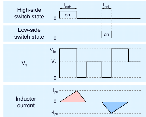
Fig. 6. Voltage and current waveforms during typical switching cycles for the switching amplifier drive stage.
