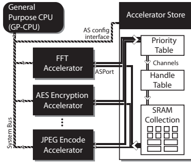
Fig. 1. Example accelerator store processor
