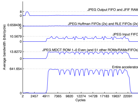
Fig. 2. JPEG accelerator memory profiles Access patterns for each accelerator memory category are shown during compression of a 640x8 pixel image. Memories within each category are similar and omitted for space.
