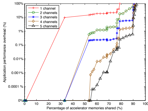
Fig. 3. Performance overhead Memories are added in order of memory selection metric. Channels represent maximum access requests from accelerators per cycle.
