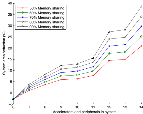
Fig. 4. System area savings System area includes accelerator store and accelerators from Table 1. GP-CPU area is considered insignificant compared to total accelerator area.
