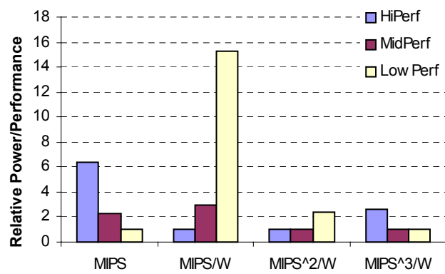
Figure 2. Relative Power-Performance
