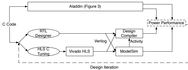
Figure 6: Validation Flow.
