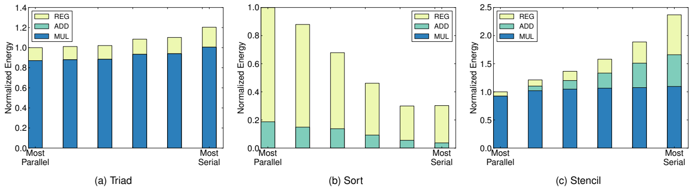
Figure 9: Energy Characterization of SHOC.
