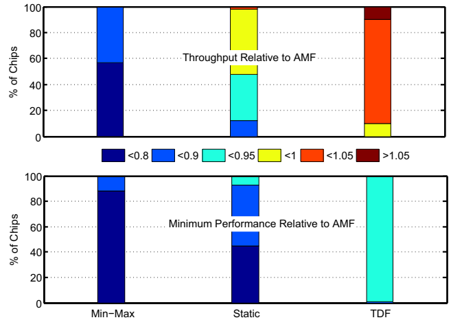
(b) Percentage of chips at various throughput & MPL relative to AMF
