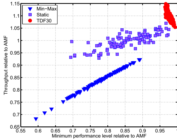
(a) Comparison of Min-Max, Static HCF & TDF
