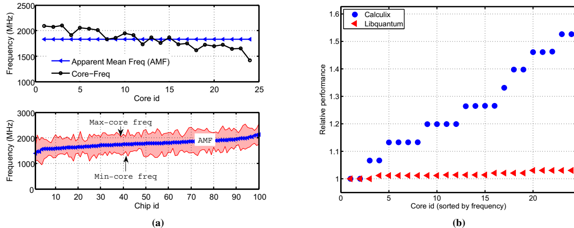
Figure 3: (a) Distribution of core frequencies on a single chip (shown in figure 2(a)) [top] and across 100 chips [bottom]. Apparent Mean Frequency (AMF) is the average frequency of the chip. (b) Performance of two applications on 24 cores normalized to their performance on slowest core: calculix (compute-bound application) is highly sensitive to the running core; libquantum (memory-bound application) exhibits smaller performance differences among cores.
