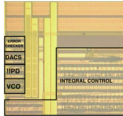
Fig. 12. Chip micrograph and performance summary table.
