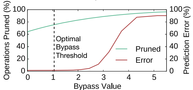
Figure 8: Analysis of neuron activities and sensitivity of prediction error to pruning. The vertical line corresponds to the point our error bound is exceeded.
